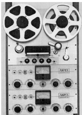
Fig. 9. Two-channel Model 351, rack mounted.
